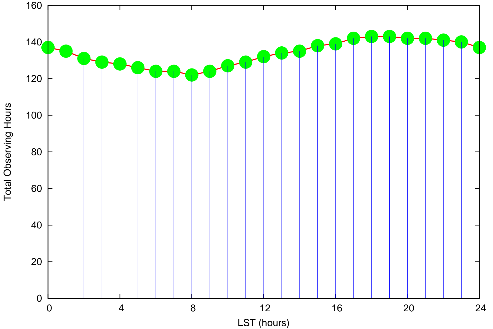
Availability of LST slots in cycle # 42, 21Apr2022 - 03Oct2022
